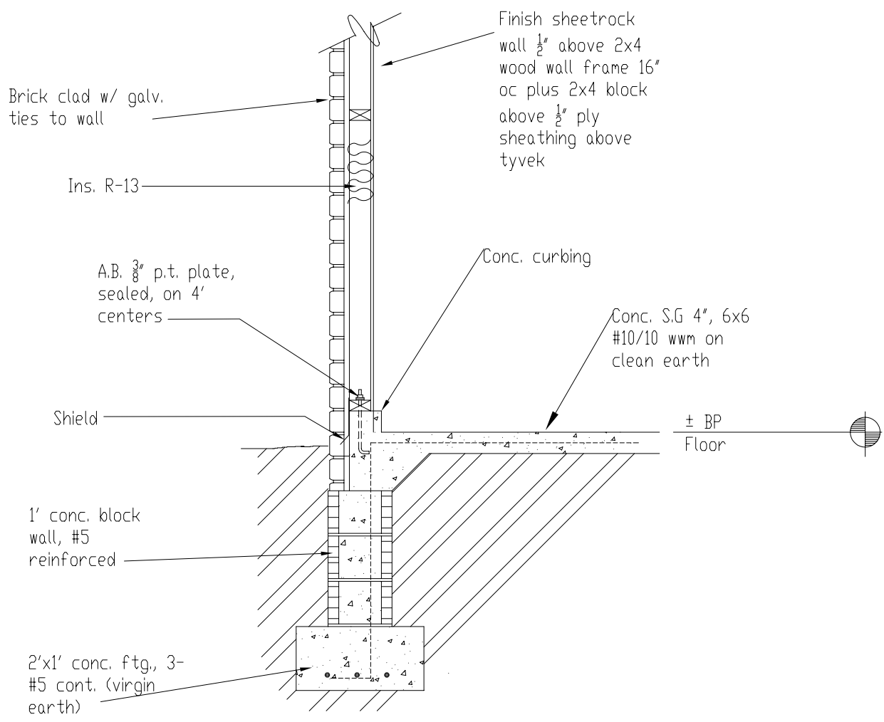
Wall Section, Garage Scale = \frac{3}{8} " to 1'
